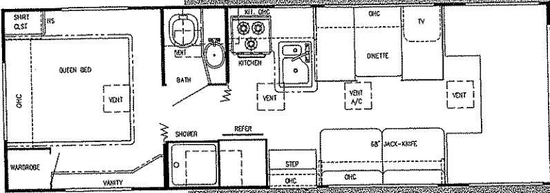
Model W6272B (Twin Beds or Bunks Opt.)
