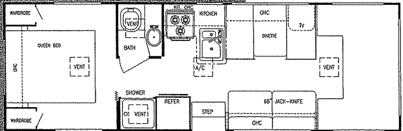
Model W6272T (Twin Beds, Slider Bed or Bunks Opt.)
