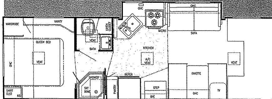
Model W6313B - Kitchen Slide-Out
