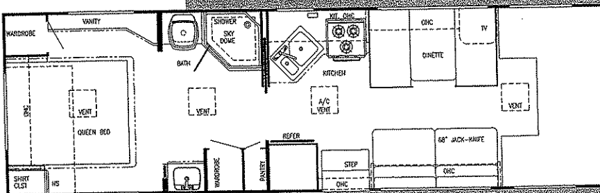
Model W6301B (Twin Beds or Bunks Opt.)
